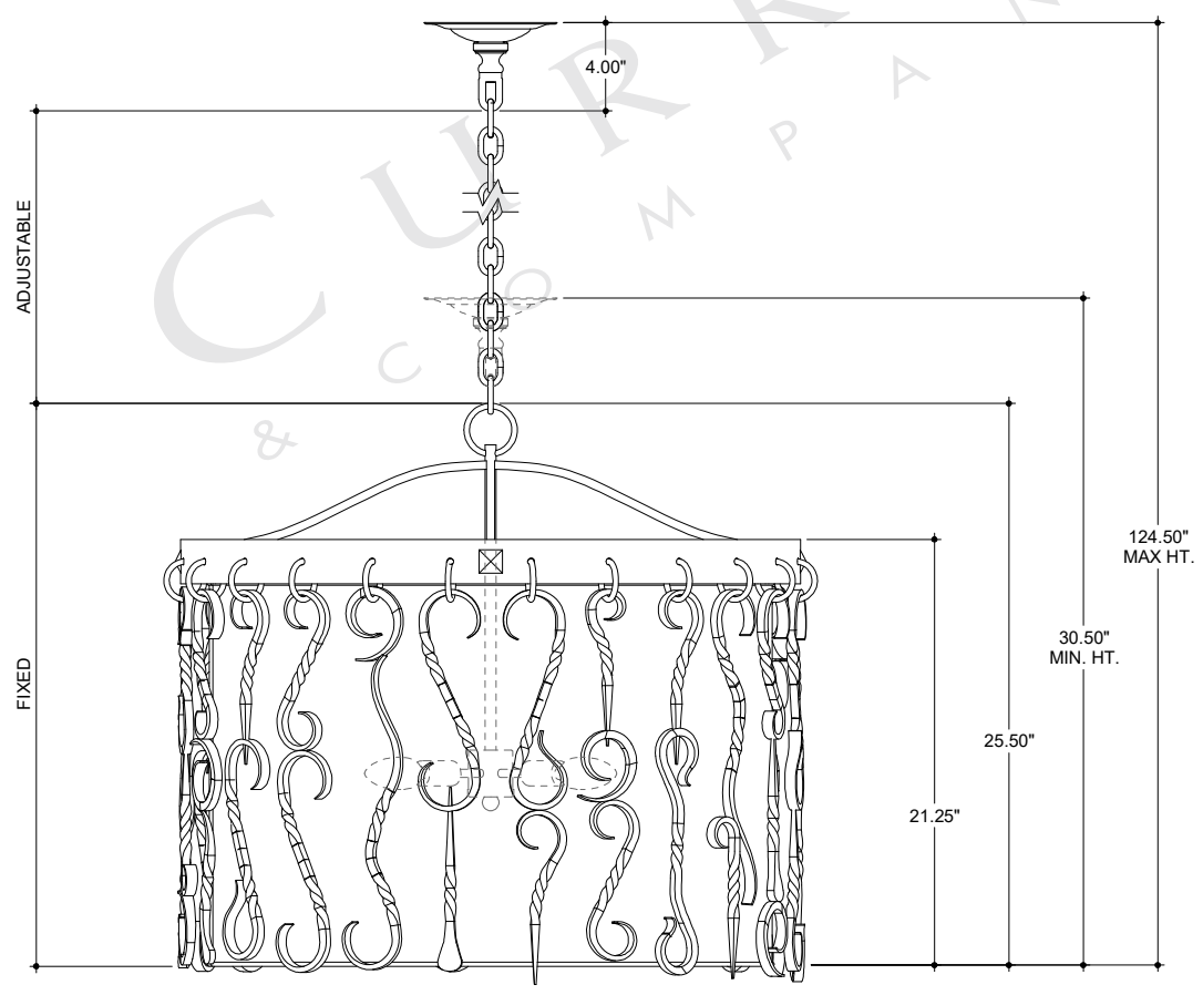
FRONT VIEW
